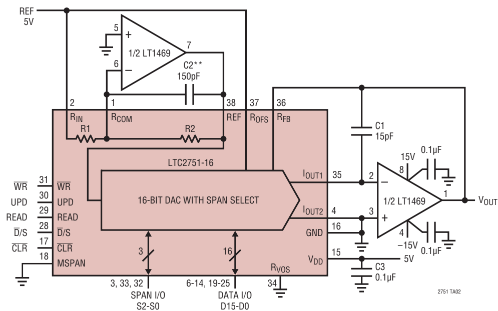
16-Bit DAC with Software-Selectable Ranges
