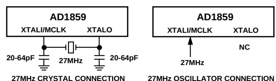
Figure 9. Crystal and Oscillator Connections
