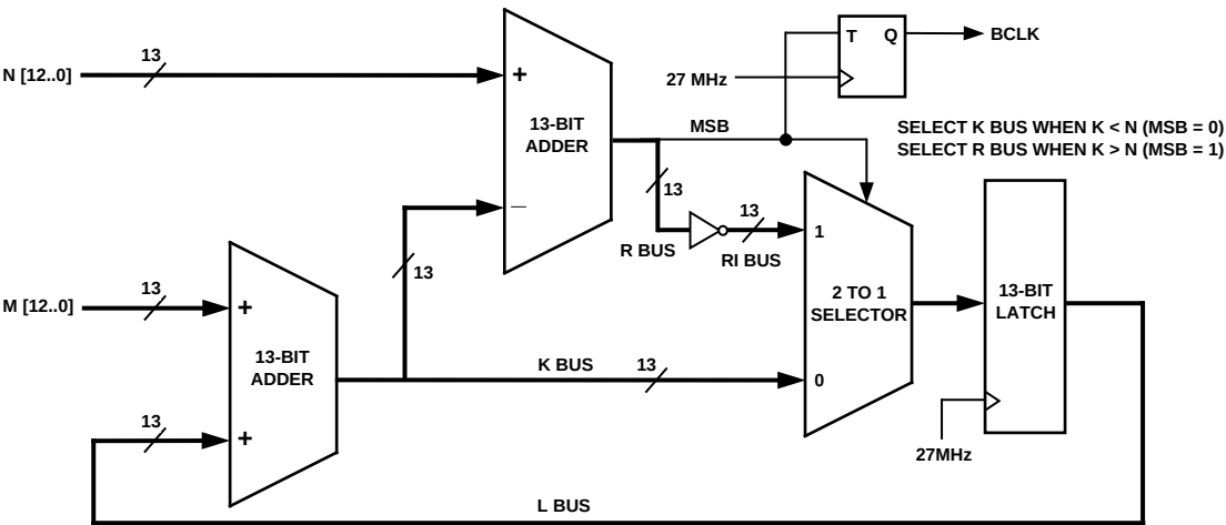
Figure 33. Numerically Controlled Oscillator Circuit
