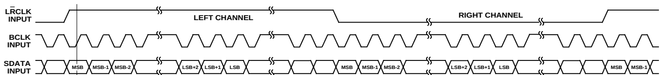
Figure 4. Left-Justified Mode
