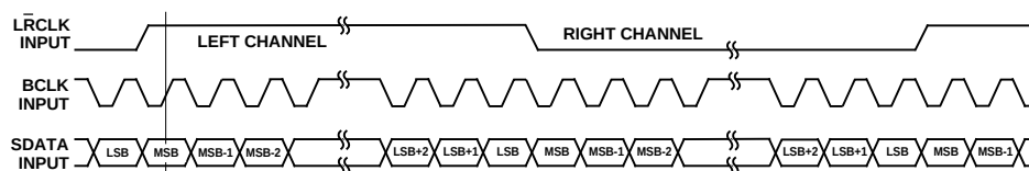
Figure 6. 32 \times F_S Packed Mode
