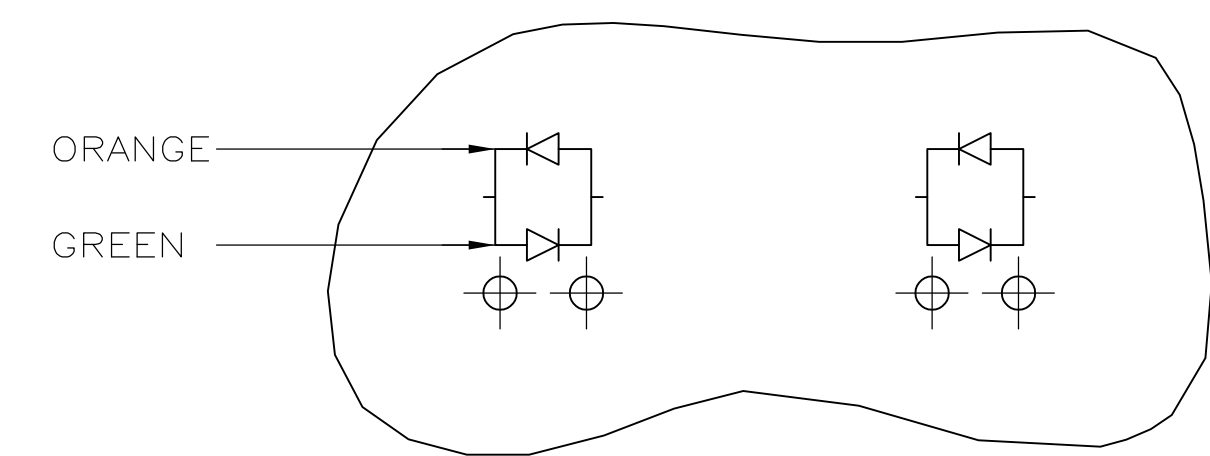
LED CURRENT DIAGRAM 7 OBSOLETE — 5406536-7 ONLY
