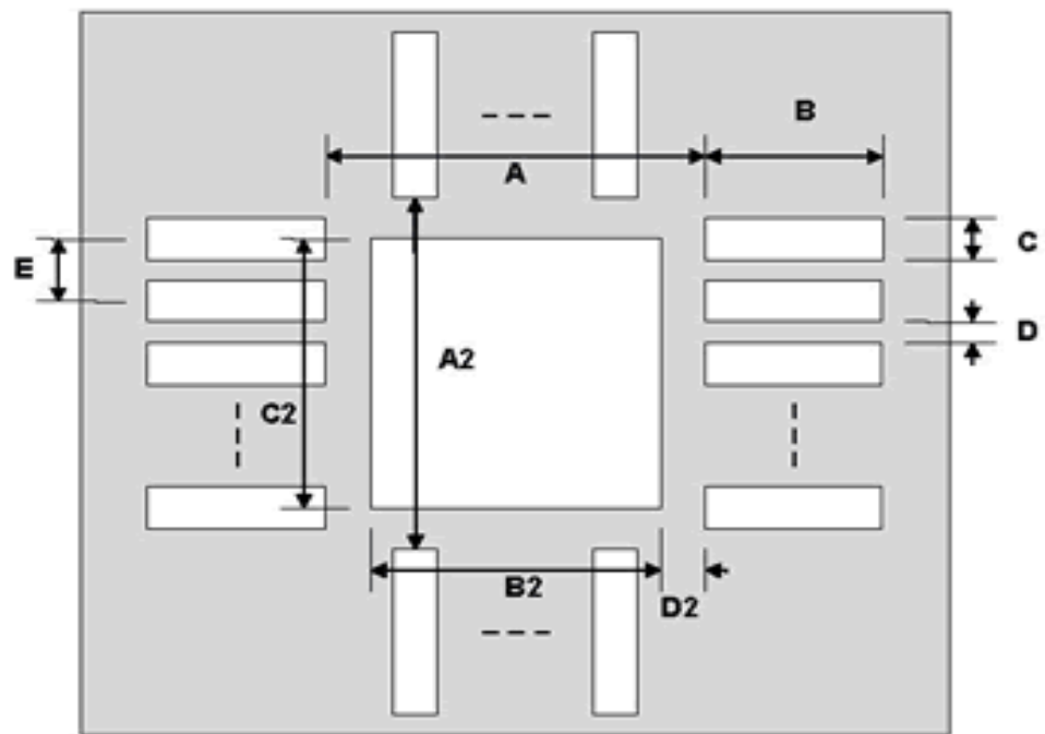
Top View (SMT Footprint)
