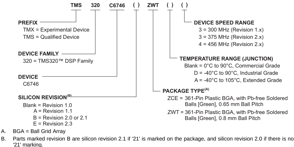
Figure 7-1. Device Nomenclature
