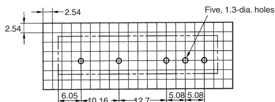
Terminal Arrangement (Bottom View)
