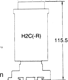
Mounting Height of Timer with Socket
