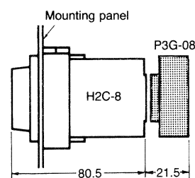
Mounting Height of Timer with Socket
