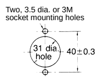
Mounting Holes
