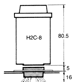
Mounting Height of Timer with Socket
