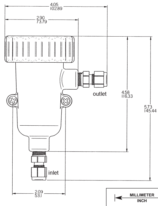
SENSOR SHOWN IN LOW FLOW CELL ASSEMBLY (PN 24091-00)
