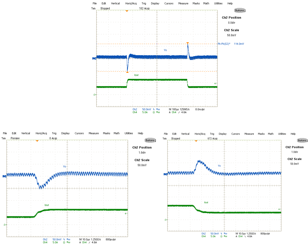
Fig. 24: Transient Response, 3A to 6A step 2.5A/ \mu s
