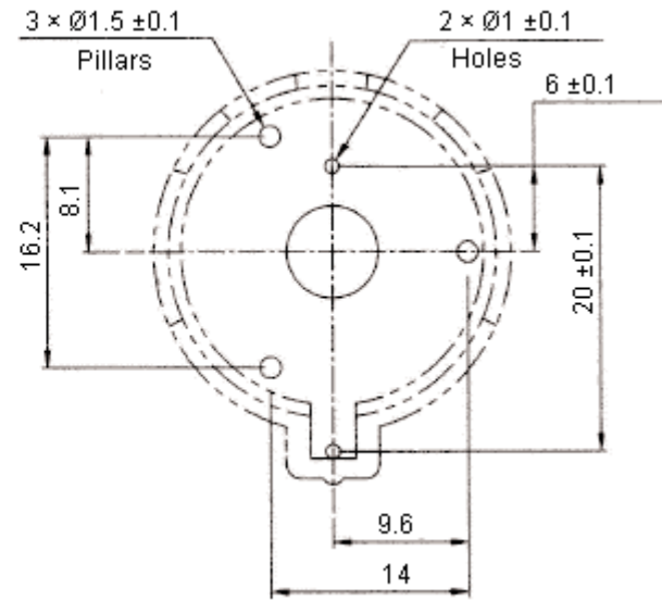
PCB Mounting Layout
