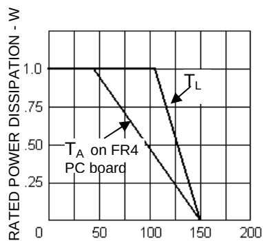
FIGURE 1 Power Derating Curve
