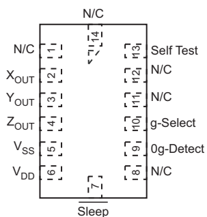
Figure 4. Pinout Description
