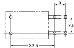
Terminal Arrangement/ Internal Connection (Bottom View)
