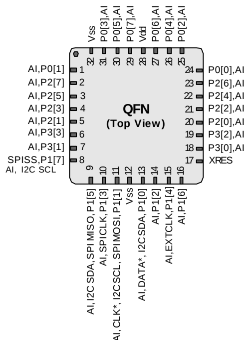
CY8C20434 32-Pin PSoC Device
