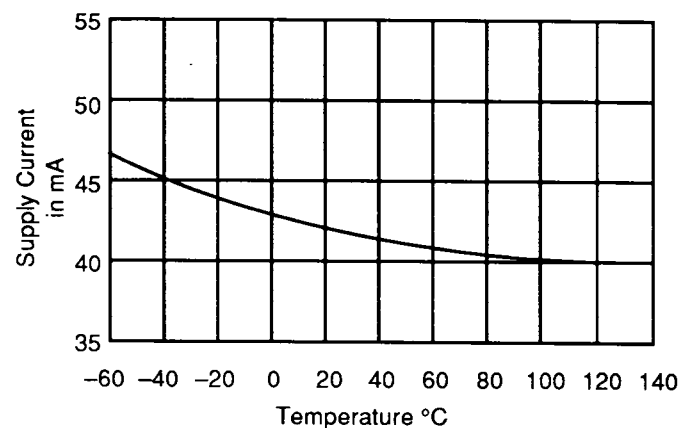
Figure 2. Typical Supply Current vs. Temperature V CC = 5.0 V, f = 10 MHz
