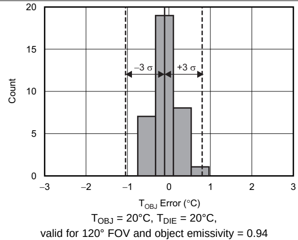
Figure 2. Typical Object Temperature Error
