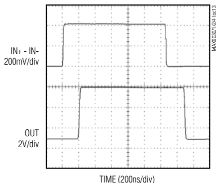
PROPAGATION DELAY
