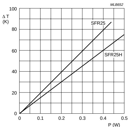
SFR25/SFR25H 5043E/5053H
