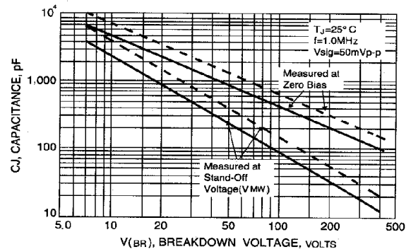
FIGURE 4 TYPICAL CAPACITANCE VS STAND-OFF VOLTAGE
