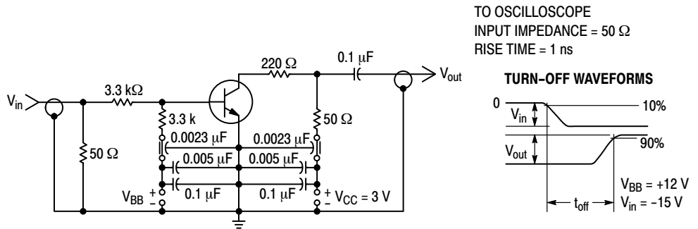
Figure 5. Turn-On and Turn-Off Time Test Circuit
