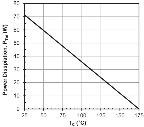
Figure 3: Power Dissipation
