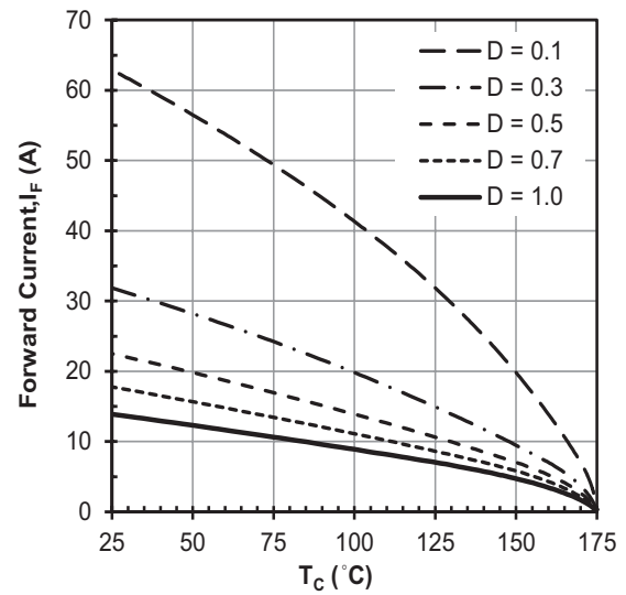
Figure 4: Diode Forward Current
