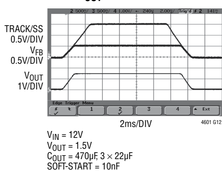
Track, I_{OUT} = 12A
