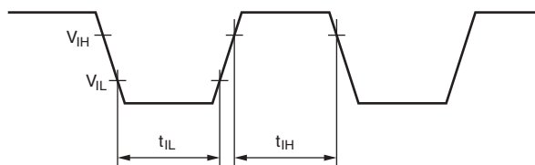
Figure 17.3 Input Timing
