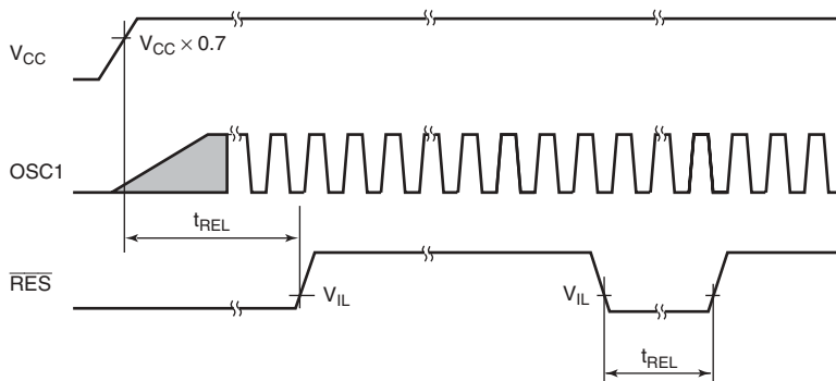
Figure 17.2 \overline{RES} Low Width Timing
