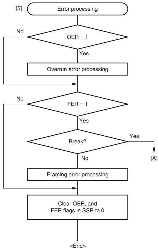
Figure 13.17 Sample Multiprocessor Serial Reception Flowchart (2)
