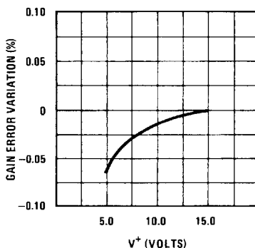
FIGURE 2. Gain Error Variation vs V^+
