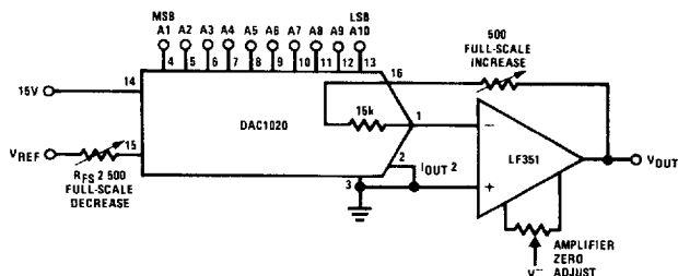
FIGURE 4. Full-Scale Adjust
