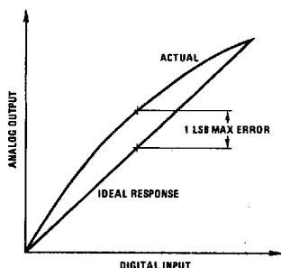
(a) End point test after zero and full-scale adjust. The DAC has 1 LSB linearity error.
