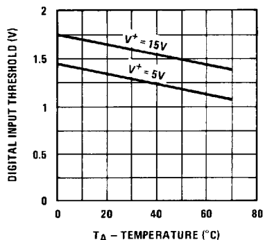
FIGURE 1. Digital Input Threshold vs Ambient Temperature
