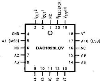
DAC1020 PLCC Package
