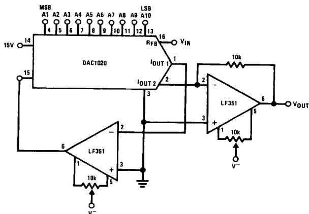
FIGURE 10. Analog-to-Digital Divider (or Digitally Gain Controlled Amplifier)
