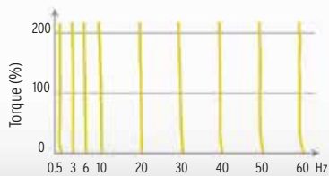
Frequency response vs Torque variation Example with 7.5 kW 4-pole motor
