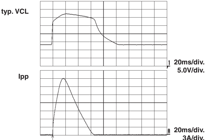
Typical Voltage and Current curve with D.U.T.
