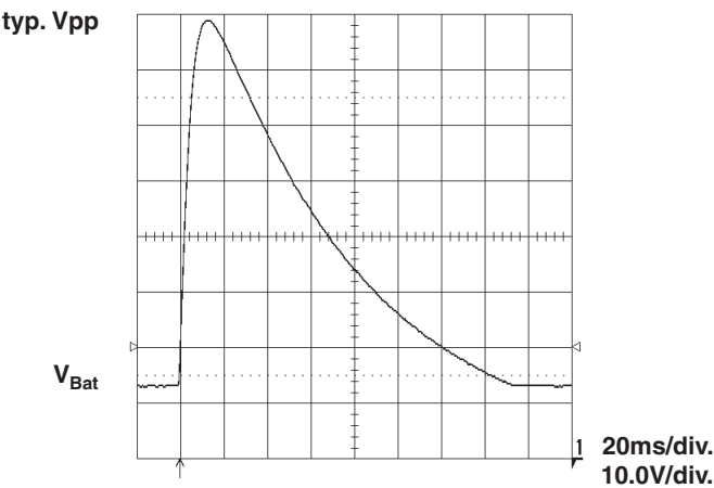
Typical Voltage curve (open circuit)
