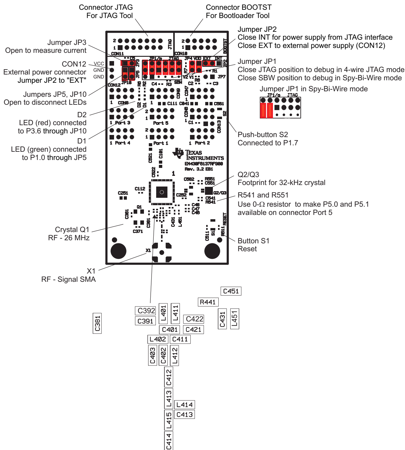
Figure B-81. EM430F6137RF900 Target Board, PCB
