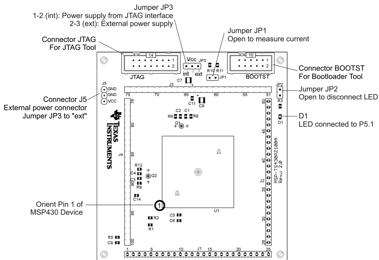
Figure B-63. MSP-TS430PZ100A Target Socket Module, PCB
