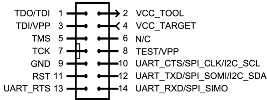
Figure B-93. JTAG Connector Pinout
