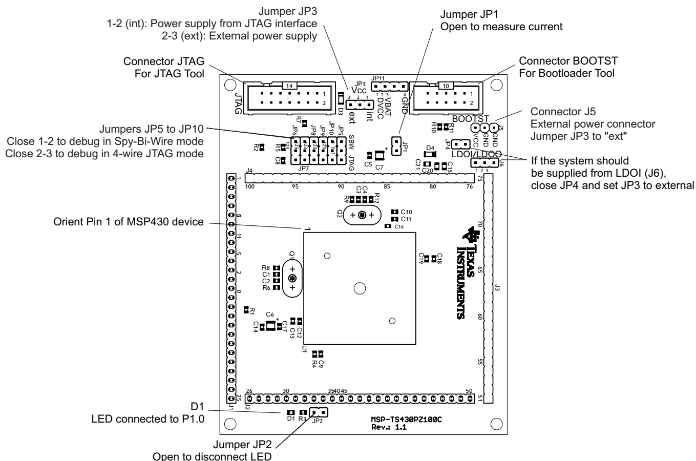
Figure B-67. MSP-TS430PZ100C Target Socket Module, PCB
