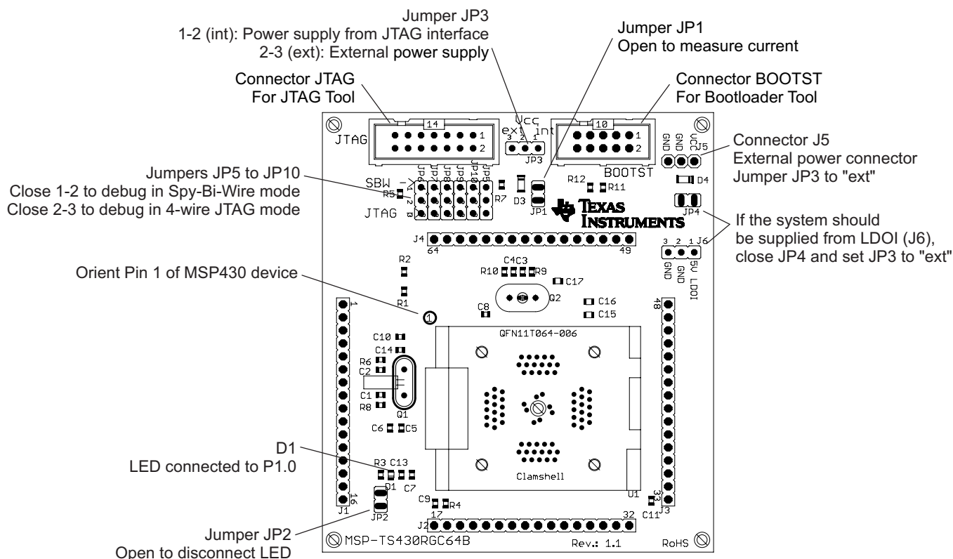
Figure B-47. MSP-TS430RGC64B Target Socket Module, PCB
