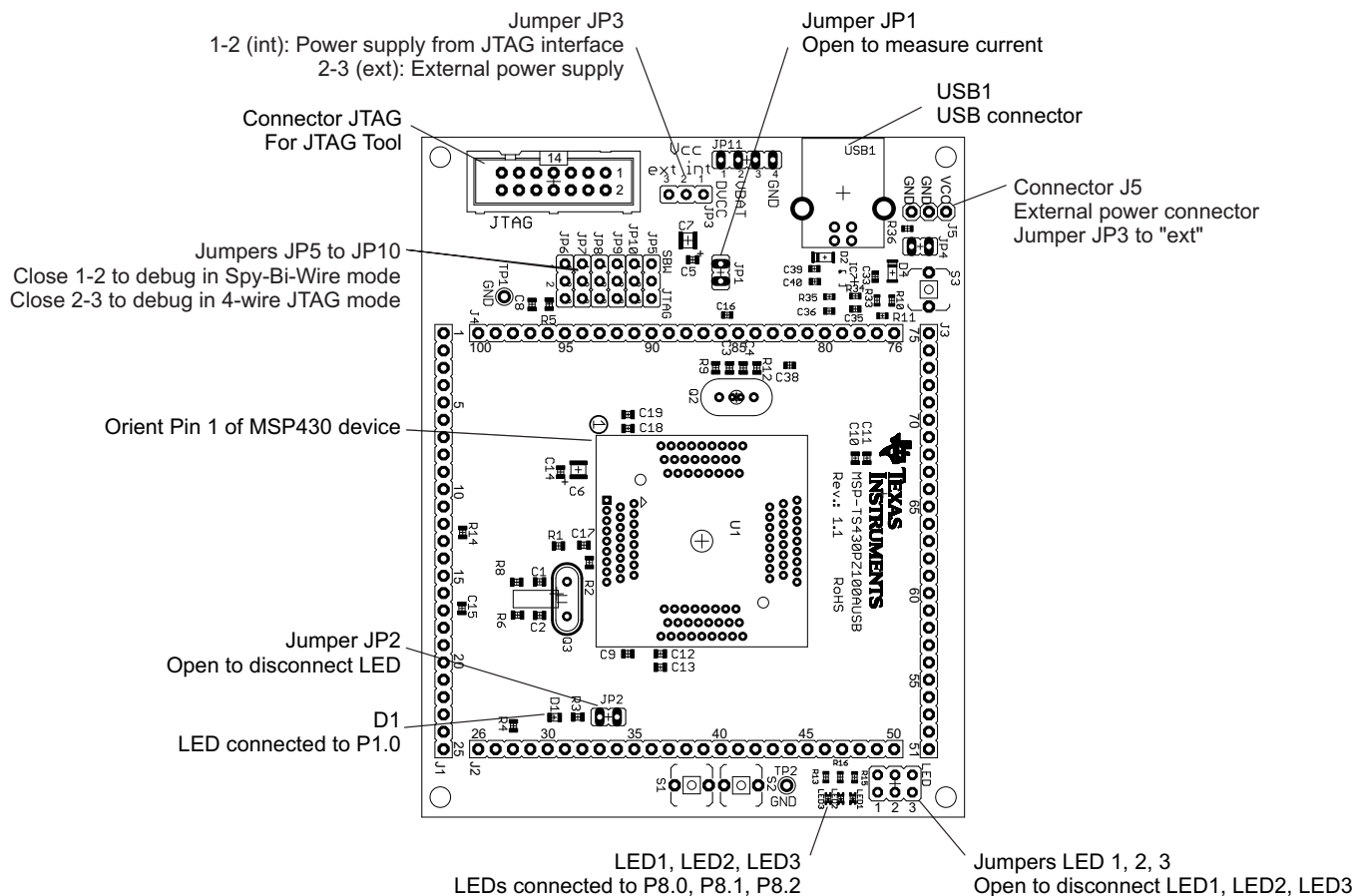
Figure B-75. MSP-TS430PZ100AUSB Target Socket Module, PCB
