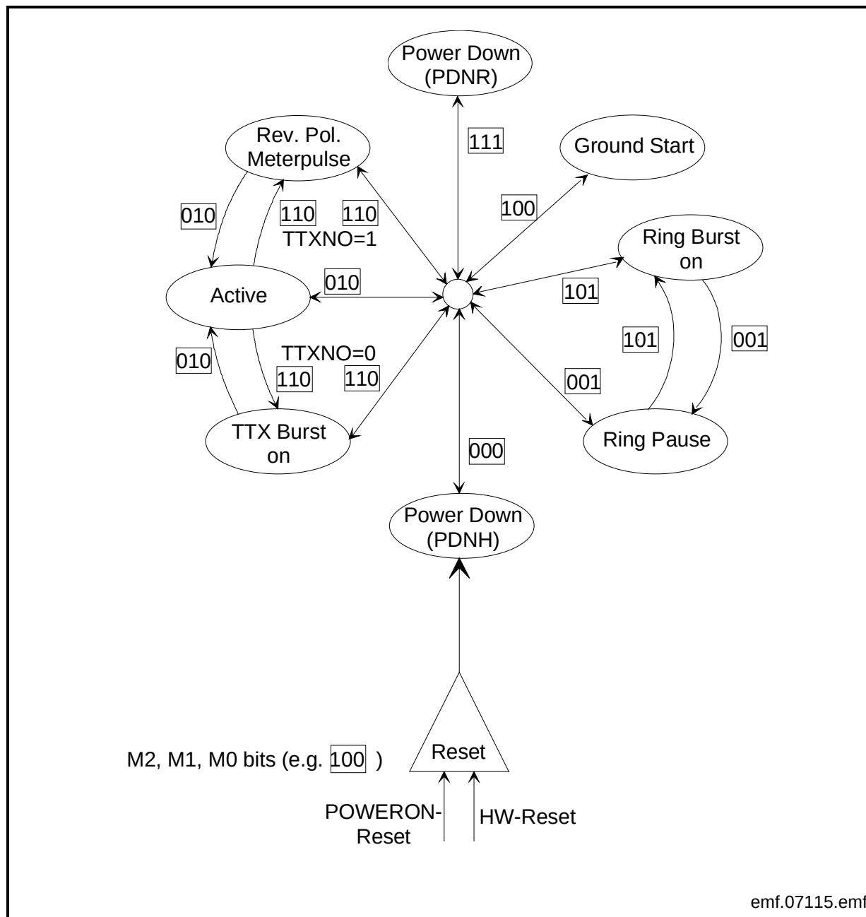
Figure 31 Operating Modes
