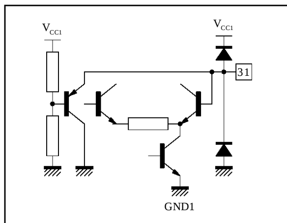
Figure 28 : Pin 31 - BCL
