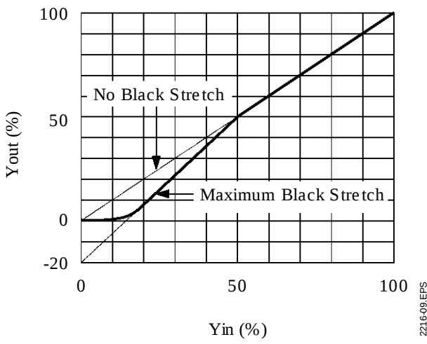
Figure 7 : Black Stretch Control
