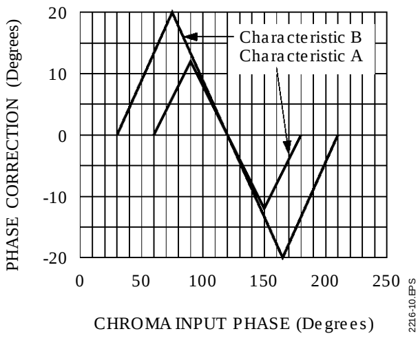
Figure 8 : Automatic Flesh Tint Control
