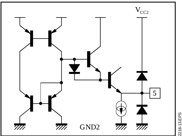
Figure 11 : Pin 5 - ACC
