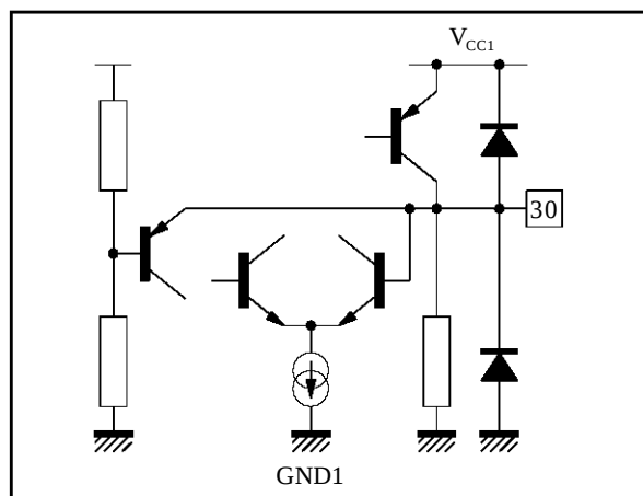
Figure 27 : Pin 30 - ICAT
