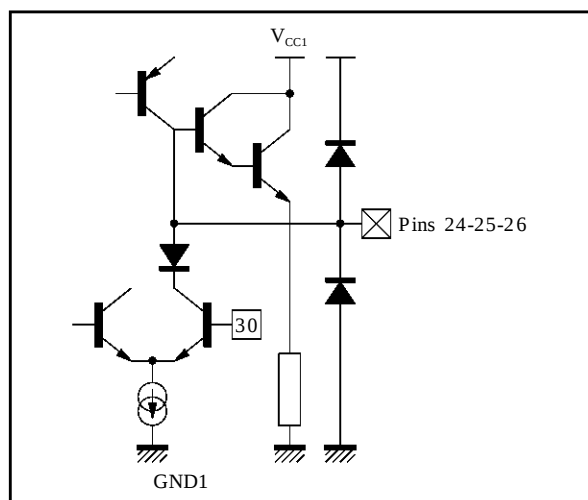
Figure 27 : Pin 30 - ICAT
