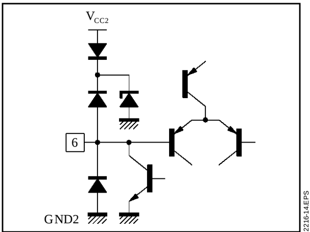
Figure 12 : Pin 6 - SDA
