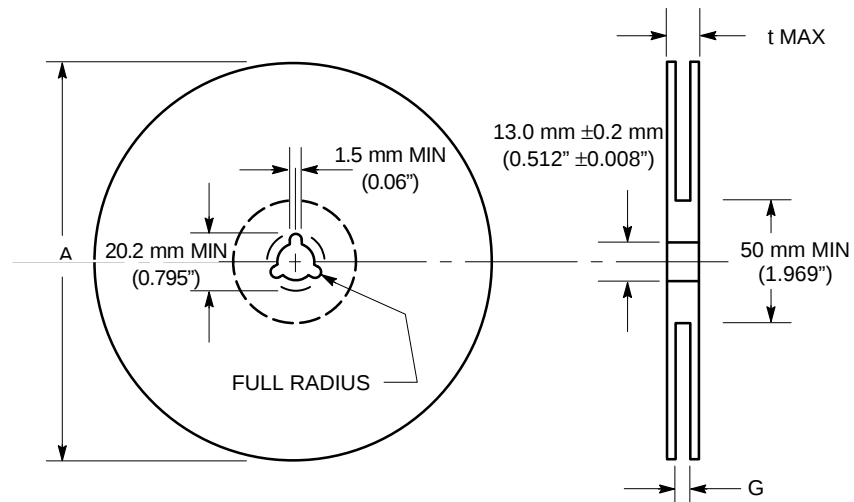
Figure 7. Reel Dimensions
