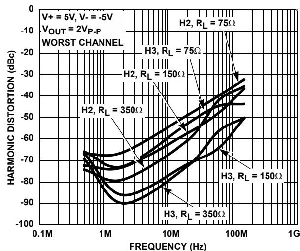
FIGURE 14. HARMONIC DISTORTION vs FREQUENCY
