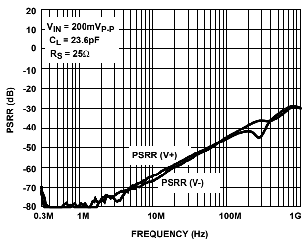
FIGURE 9. PSRR CHANNELS
