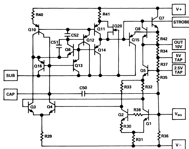
Figure 3. Schematic Diagram
