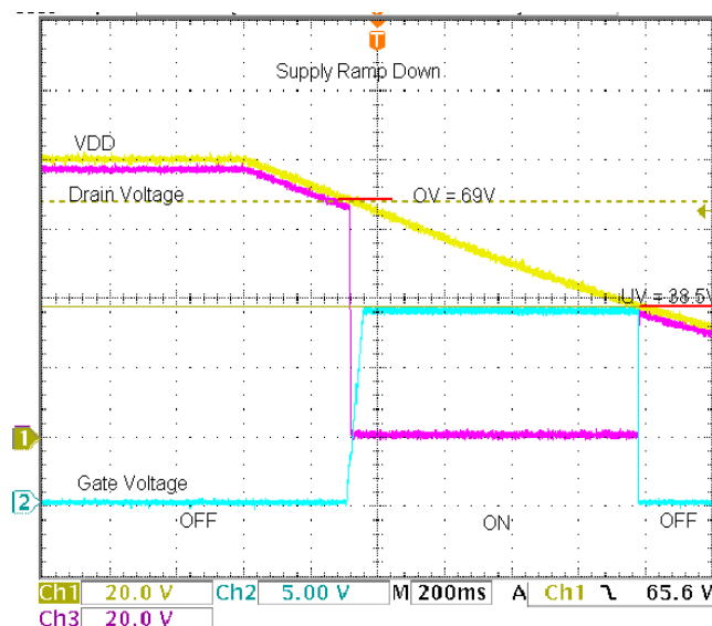
FIGURE 29. SUPPLY RAMP-DOWN
