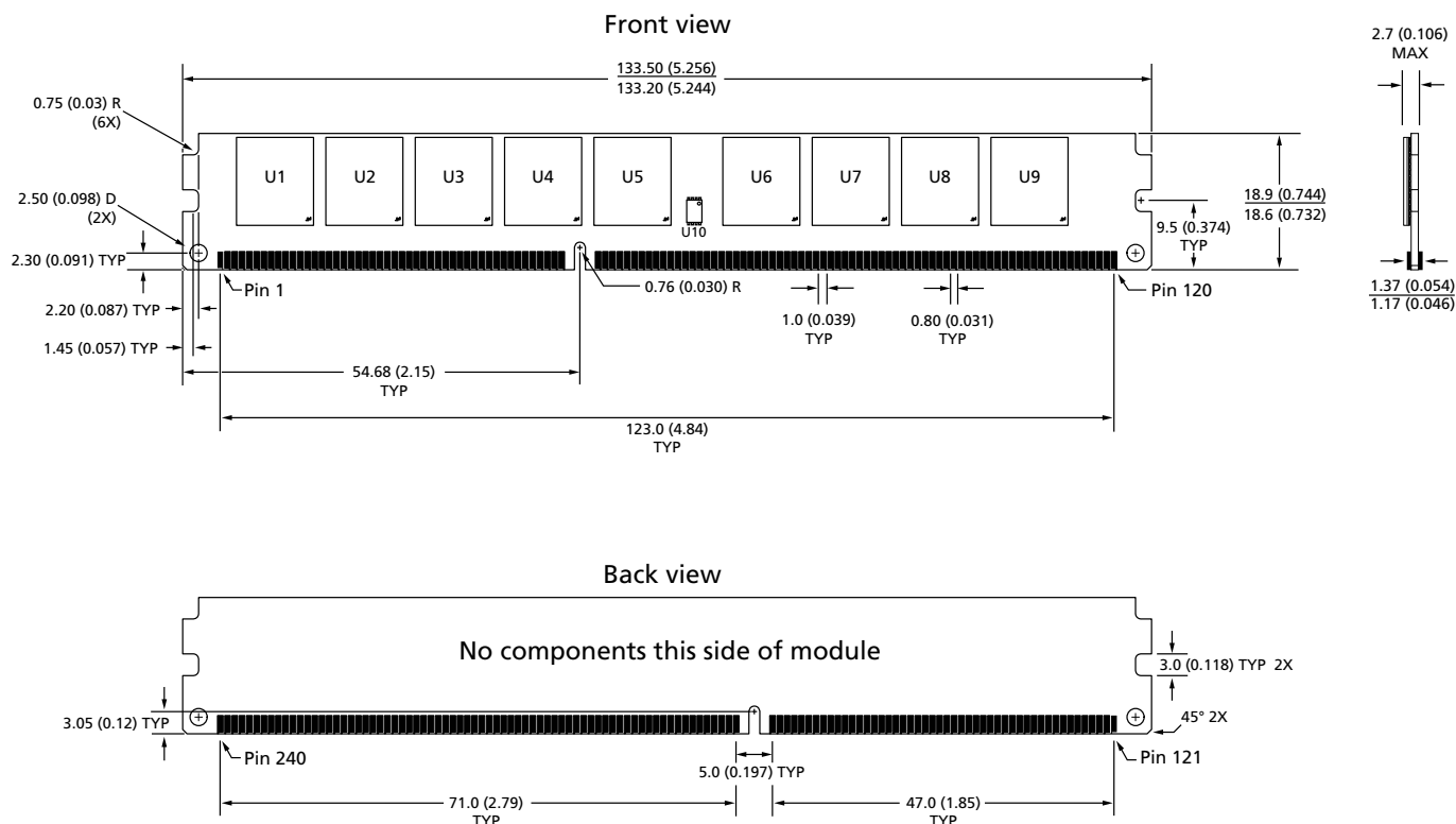
Figure 3: 240-Pin DDR3 UDIMM
