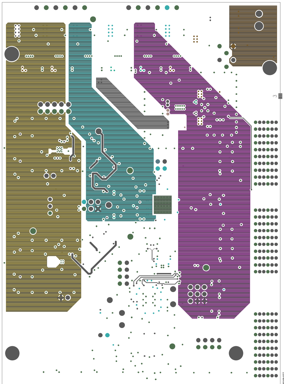
Figure 28. Power Plane (Layer 3)
