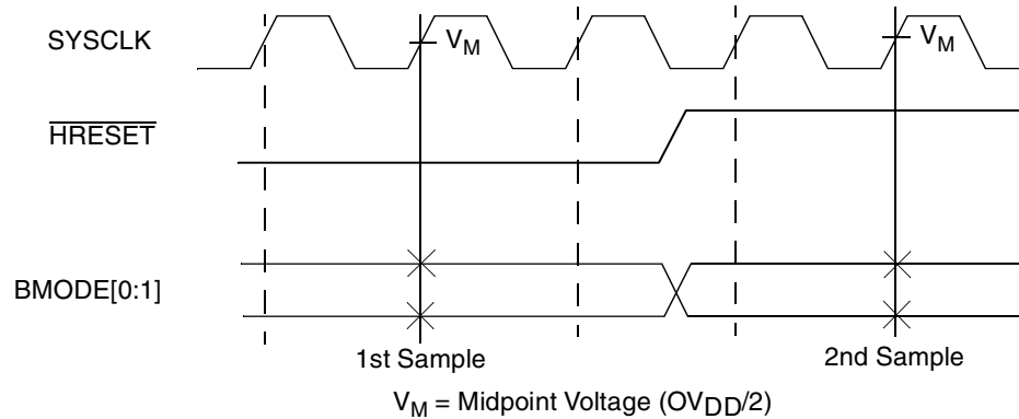
Figure 5. \overline{BMODE}[0:1] Input Sample Timing Diagram
