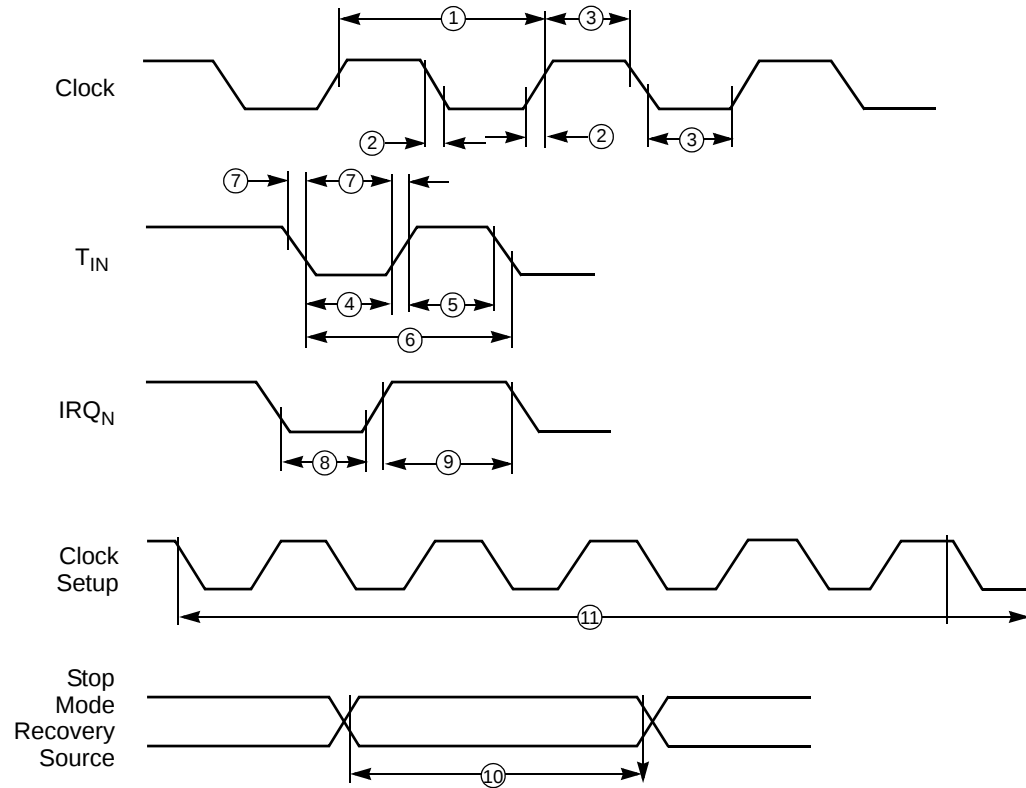
Figure 5. Timing Diagram
