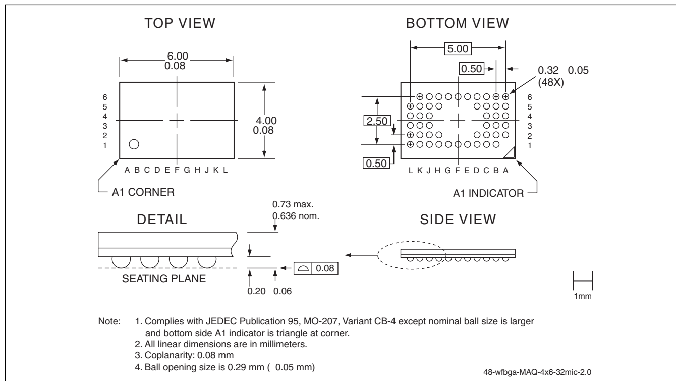
FIGURE 25: 48-Ball Very-Very-Thin-Profile, Fine-Pitch Ball Grid Array (WFBGA) 4mm x 6mm SST Package Code: MAQ
