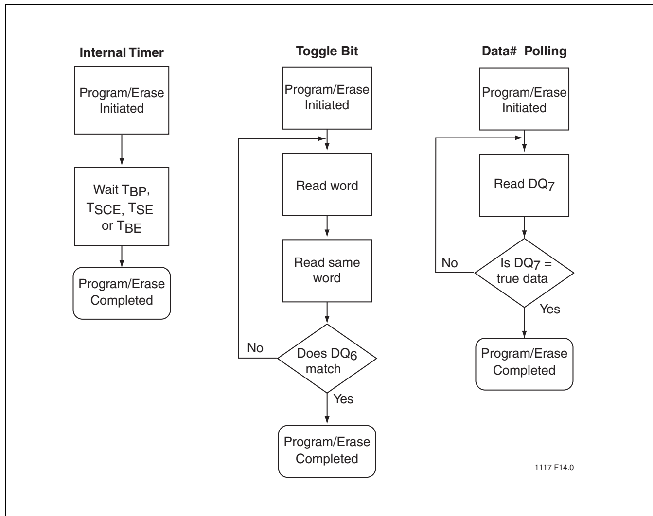
FIGURE 19: Wait Options
