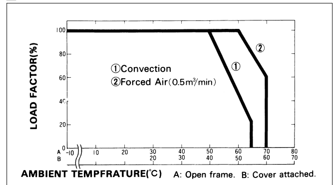
■ DERATING CURVE
