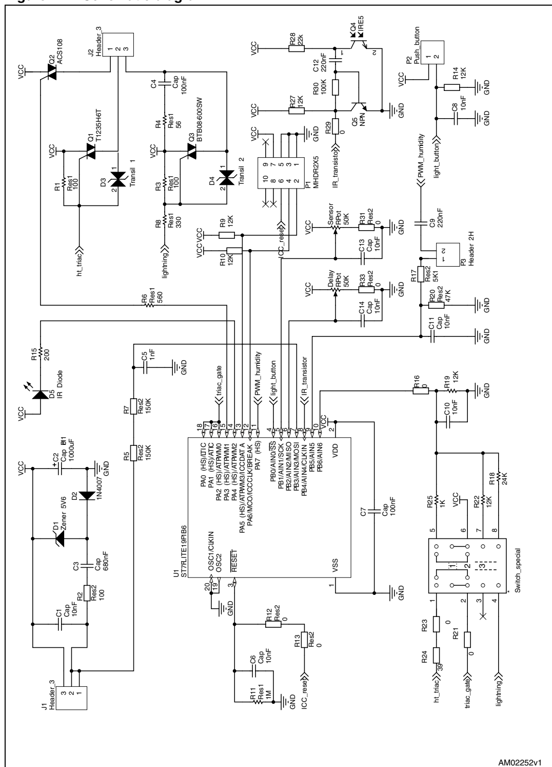
Figure 1. Schematic diagram
