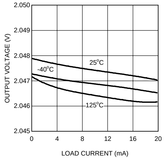
Figure 18. Load Regulation
