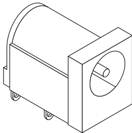
16PJ031 A=ø2.0mm.004 16PJ032 A=ø2.35mm.004
