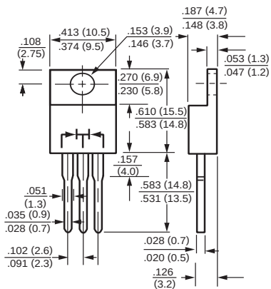
TO-220
