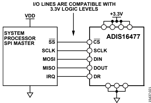
Figure 19. Electrical Connection Diagram
