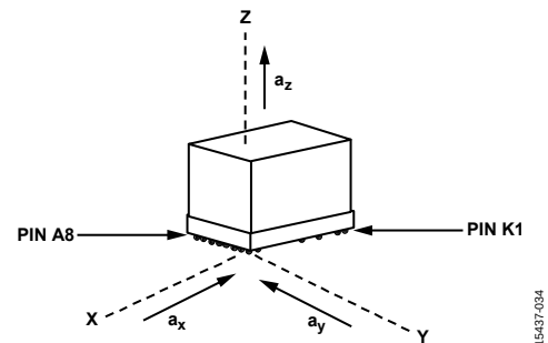
Figure 32. Accelerometer Axis and Polarity Assignments
