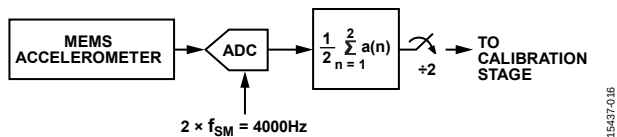
Figure 14. Accelerometer Data Sampling
