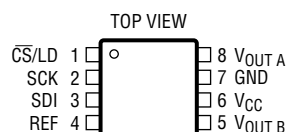
MS8 PACKAGE 8-LEAD PLASTIC MSOP T_{JMAX} = 125^{\circ}\text{C} , \theta_{JA} = 300^{\circ}\text{C/W}
