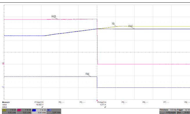
Figure 50. Overvoltage
