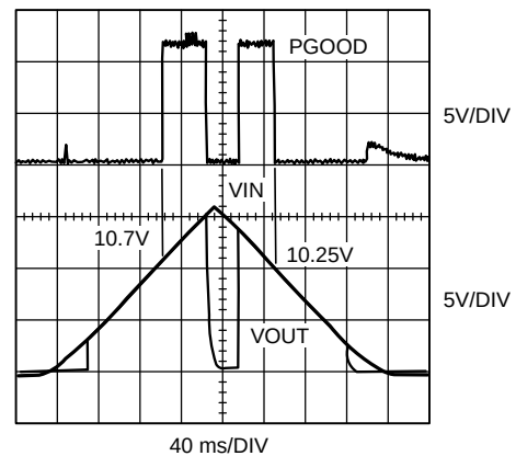
Figure 25. Start-up (PGOOD)
