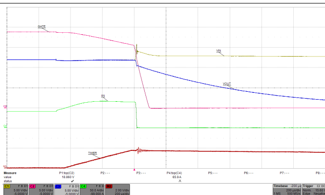
Figure 52. Loadstep
