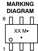
SOT-363/SC-88/ SC70-6 CASE 419B
