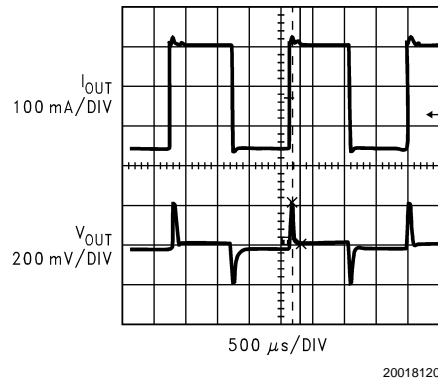
FIGURE 6. 130mA to 400mA Transient Response of the circuit in Figure 10 with C_{\text{FF}} = 1\text{nF}
