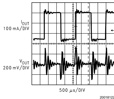
FIGURE 7. 130mA to 400mA Transient Response of the circuit in Figure 10 with C_{\text{FF}} disconnected
