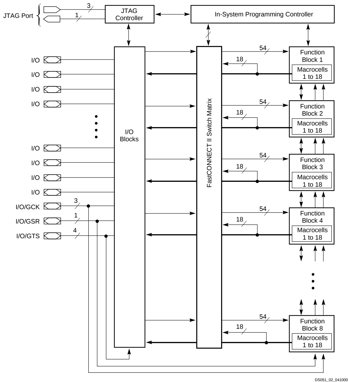
Figure 2: XC95144XV Architecture
