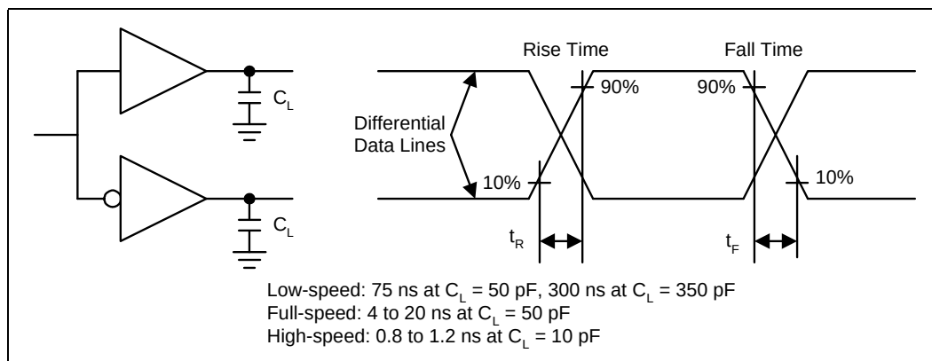
Figure 35. USB Jitter
