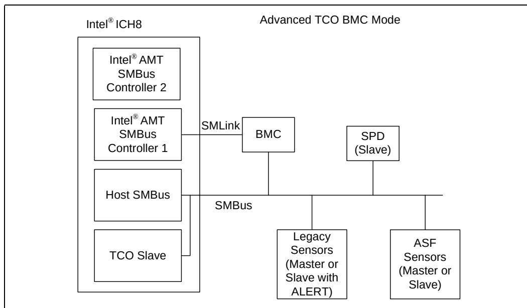
Figure 12. Advanced TCO BMC Mode SMBus / SMLink Configuration
