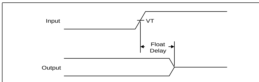
Figure 26. Pulse Width
